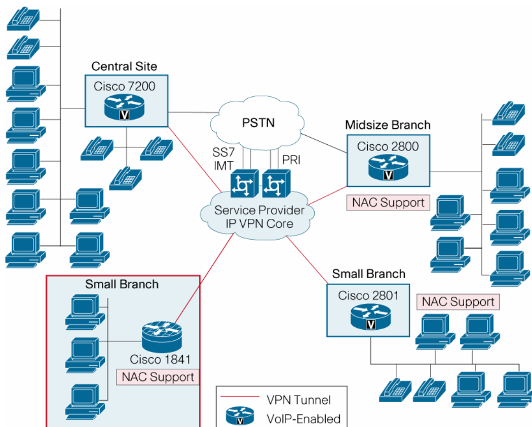
Figure 2. Secure Network Connectivity with Cisco 1841 Router
